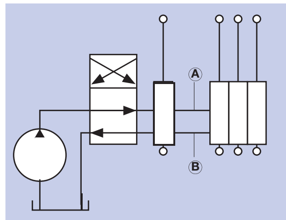
Schematic Two-line System
